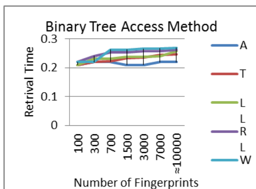
Figure 2. Results of testing binary tree
