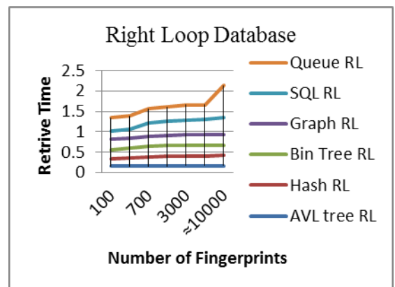
Figure 10. Time retrieve for Right Loop Class using different access methods
