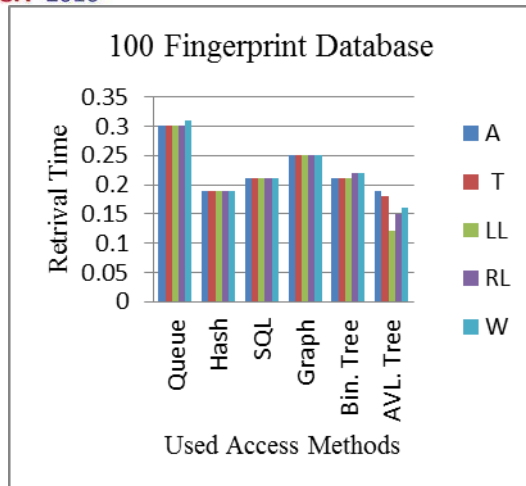
Figure 1. Time retrieval from 100 Fingerprint Database
