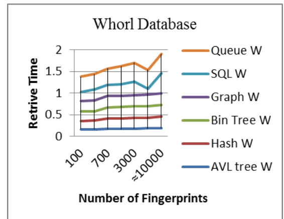
Figure 9. Time retrieve for whorl Class using different access methods
