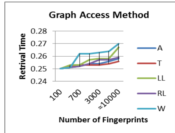
Figure 3. Results of testing graph method
