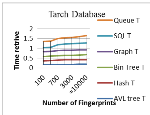
Figure 7. Time retrieve for Tarch Class using different access methods
