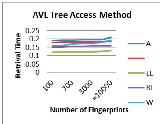
Figure 6. Results of testing AVL tree method
