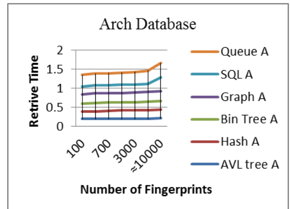
Figure 8. Time retrieve for Arch Class using different access methods
