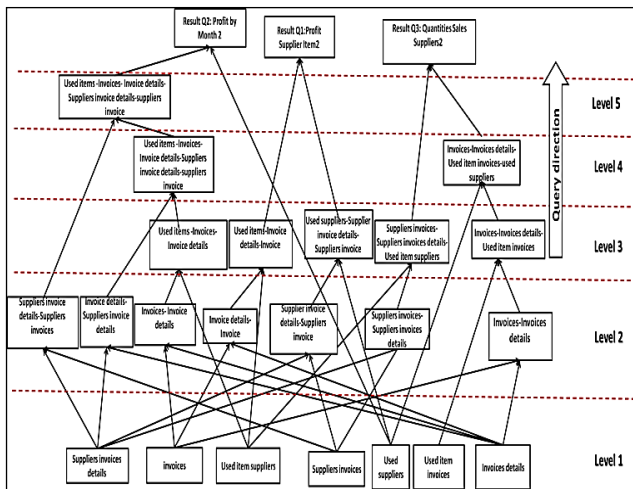
Figure 5. Lattice illustrates the levels of query optimization after using MV.
