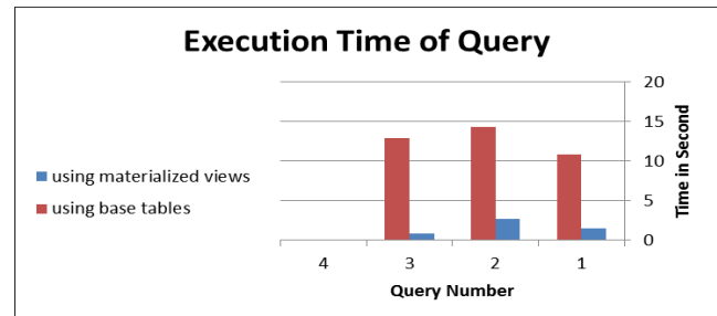
Figure 3. Difference query execution time.
