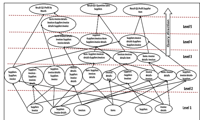
Figure 4. Lattice illustrates the levels of query optimization before using MV.
